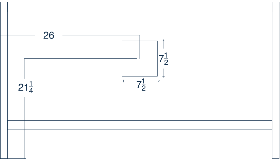
BACK VIEW (no counter top)
