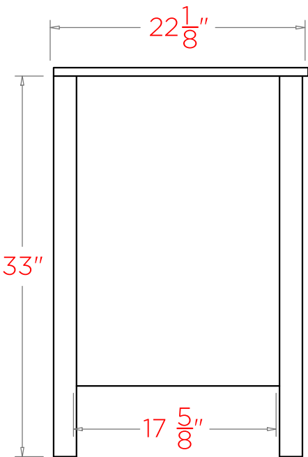
SIDE SECTION
