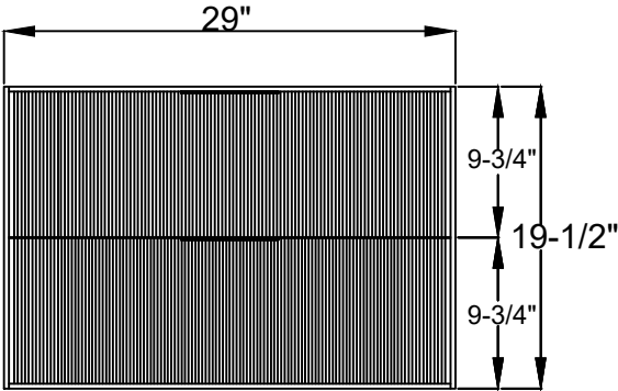
FRONT VIEW (no counter top)
